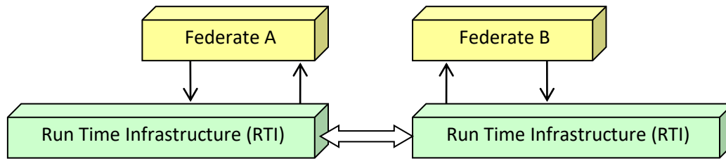
Figure 9: HLA Interaction Overview
