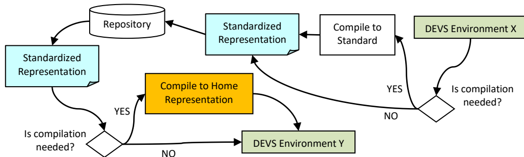
Figure 18: Standardized Model Representation Flow
