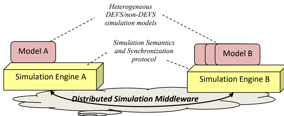
Figure 2: Concept of Standardized Distributed simulation Middleware
