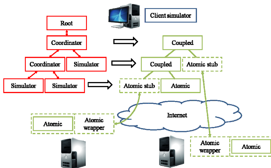
Figure 15: Local simulation of distant and local models
