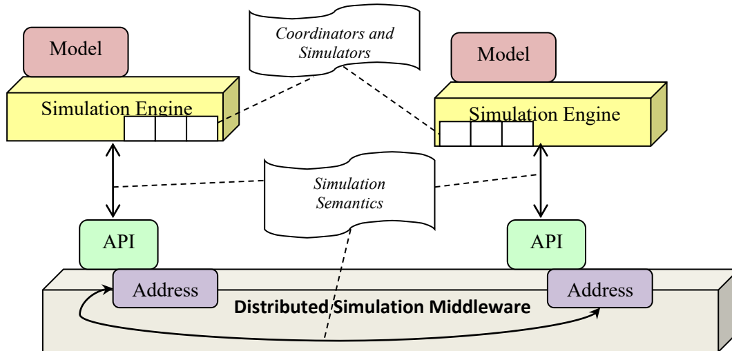
Figure 19: Standardized Middleware Reference Model
