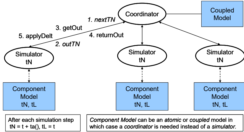
Figure 4: Abstract parallel DEVS simulator protocol
