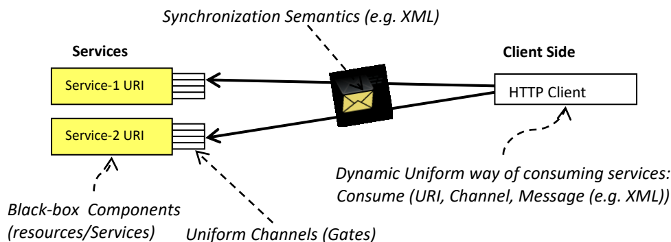
Figure 13: RESTful Web-service Client/Server Architecture
