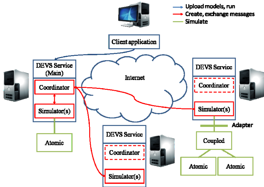
Figure 16: DEVS components interoperability through simulators communication
