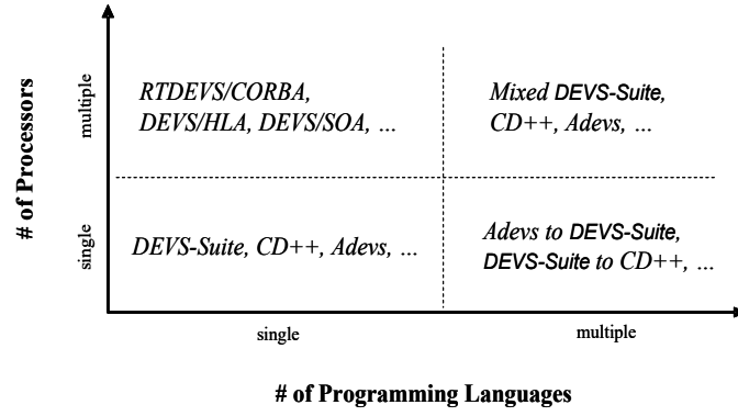
Figure 3: Centralized and distributed DEVS-based simulators
