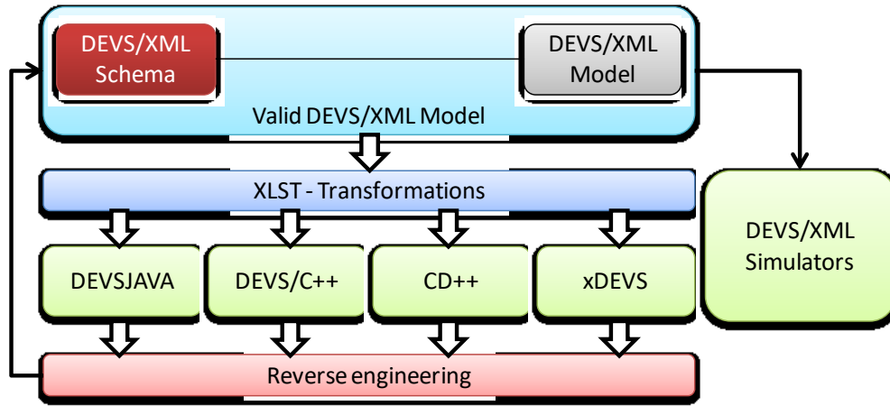
Figure 17: DEVS/XML standard definition
