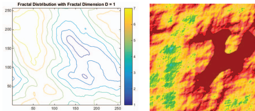
Figure 10: (a) Contour figure of the D_\rho = 1 fractal distribution D_{strength}=2.1 , (b) end of simulation.
