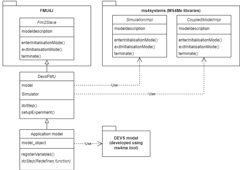
Figure 4: Design of DEVS model export.
