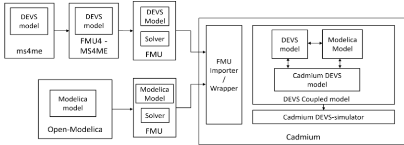
Figure 1: Block diagram for High-level overview of co-simulation in Cadmium.
