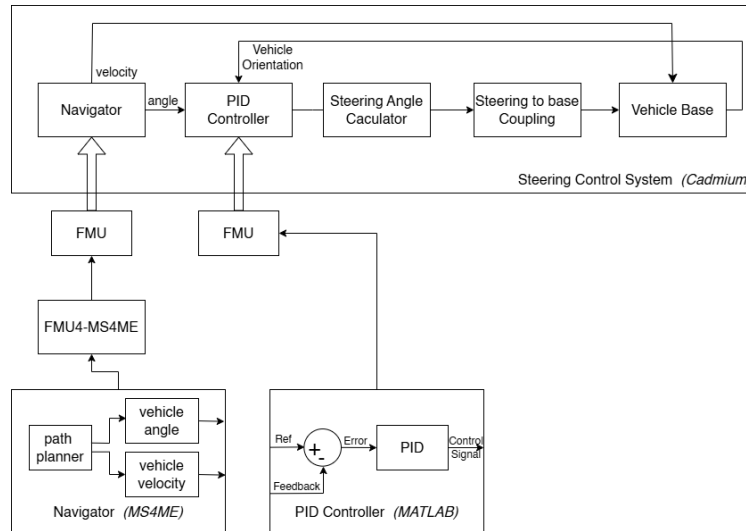
Figure 5: Steering Control System in Cadmium.
